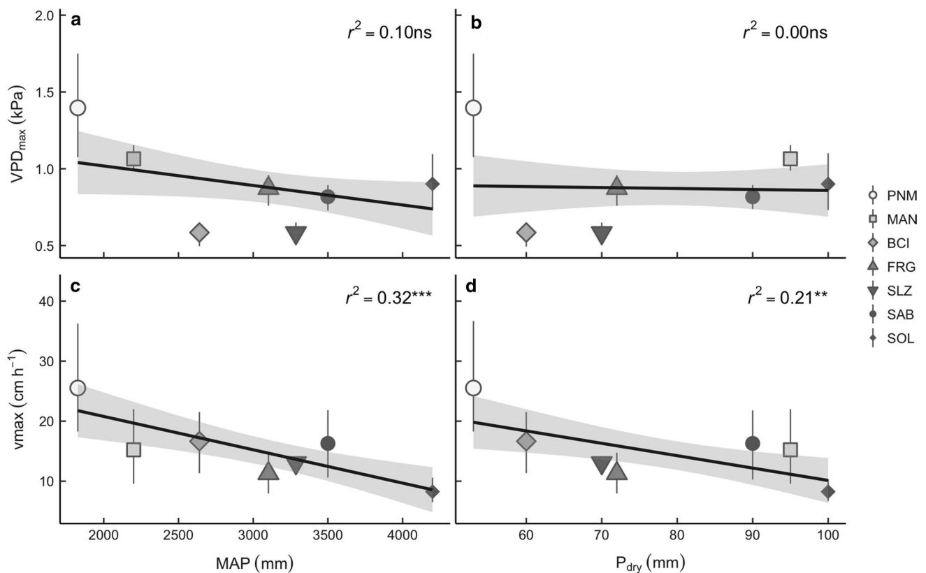
Fig. 3 Relationships between the VPD threshold at which sap flux levels-off at maximum levels ( VPD_{\max} \pm SD , kPa) and maximum sap flux ( v_{\max} \pm SD , \text{cm h}^{-1} ), and mean annual precipitation (MAP, mm)
